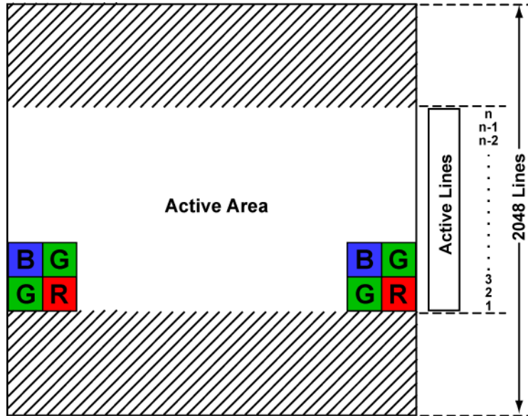
FIGURE 47. Bayer 1
